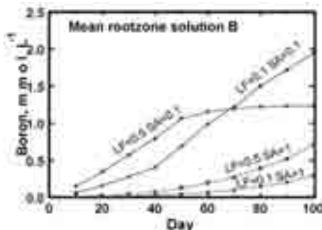
Fig. 6 Mean root zone soil solution B concentration with time as related to leaching fraction (LF) and soil surface area (SA), expressed in 10^3 \times \text{m}^2 \text{g}^{-1} (Suarez, 2002).
