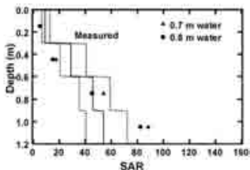
Fig. 9 Comparison of measured and model predicted changes in SAR with depth after mixing 24 Mg/ha gypsum into the top 15 cm and then infiltration of 70 or 80 cm of water. Symbols represent simulation values for the 30 cm depth intervals (Suarez, 2001).
