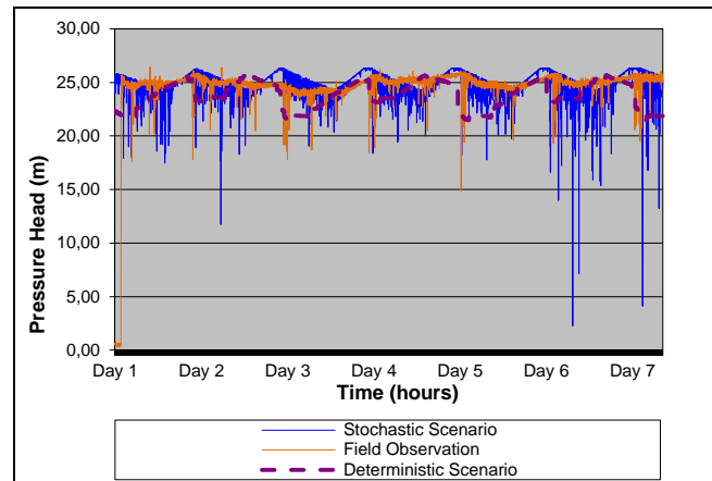
Figure 4. Comparing the pressures recorded at node 165 with the values from the models
