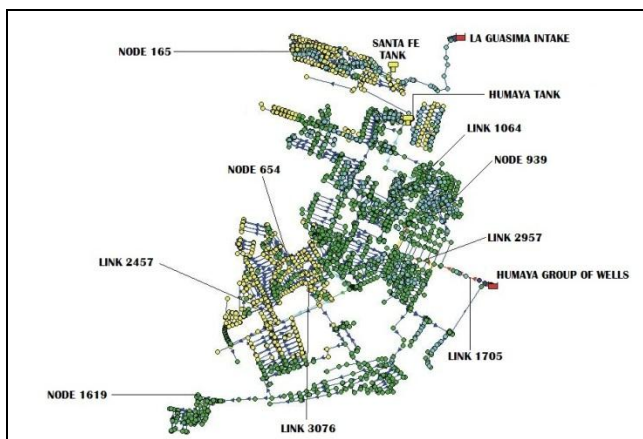
Figure 1. Location of the network of nodes and links analysed here
