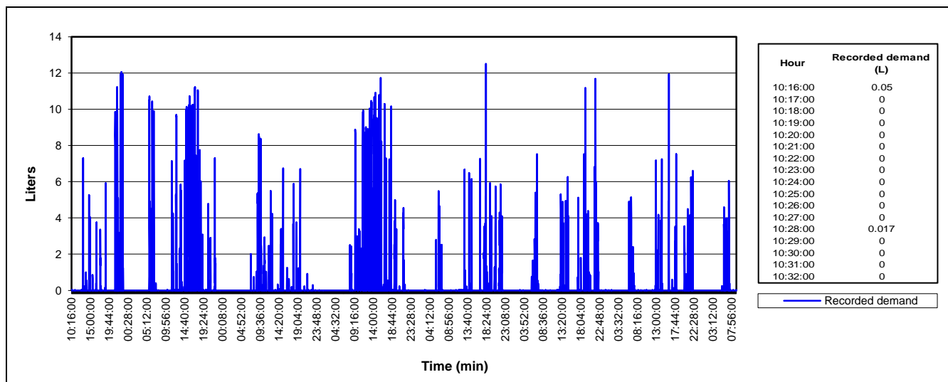
Figure 3. Recorded water demand at a home, in tabular and graphical form
