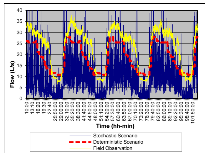
Figure 5. Comparing the measured flow rate with the HDVC and the stochastic models at link 2957
