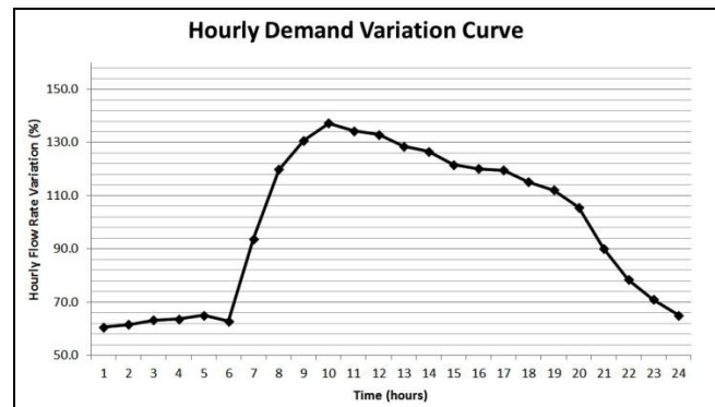
Figure 2. Hourly demand variation curve for all of Mexico (Tzatchkov 2007)
